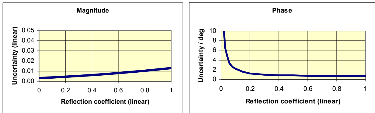
Typical accuracy of reflection magnitude and reflection phase measurements of the R&S®ZVA8 in the frequency range 1 MHz to 8 GHz, of the R&S®ZVA24 in the frequency range 50 MHz to 24 GHz, of the R&S®ZVA40 in the frequency range 50 MHz to 40 GHz, of the R&S®ZVA50 in the frequency range 50 MHz to 50 GHz and of the R&S®ZVA67 in the frequency range 50 MHz to 67 GHz.
