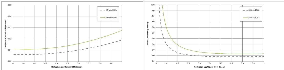
Typical accuracy of reflection magnitude and reflection phase measurements for the R&S®ZNLE3 in the frequency range from 1 MHz to 3 GHz, for the R&S®ZNLE6 in the frequency range from 1 MHz to 6 GHz. Analysis conditions: S_{12} = S_{21} = 0 , cal. power -10 dBm, meas. power -10 dBm.
