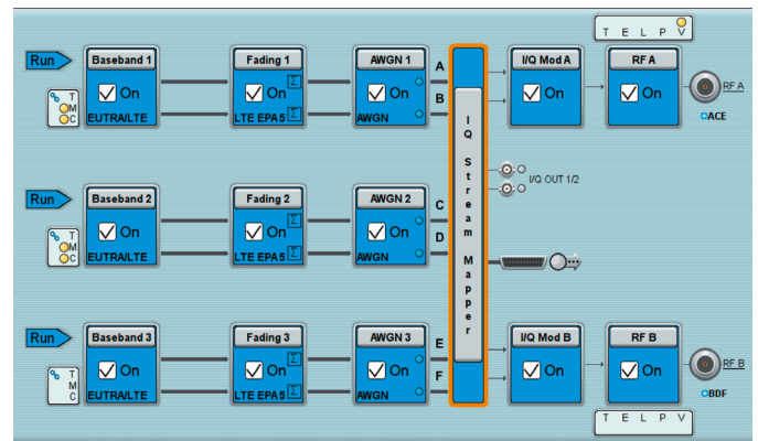
Block diagram of the R&S®SMW200A configured for the generation of a LTE Release 11 fciC test scenario. One R&S®SMW200A simultaneously generates the LTE serving cell as well as the two aggressor cells, each with 2x2 MIMO, with correlated fading channels.
