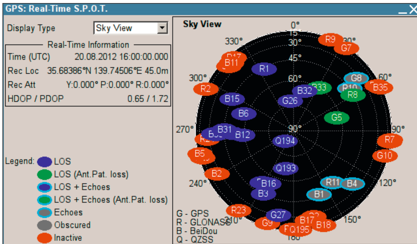
Simulation of a combined GPS/Glonass/Galileo/BeiDou/QZSS constellation with consideration of signal obscuration and multipath.
