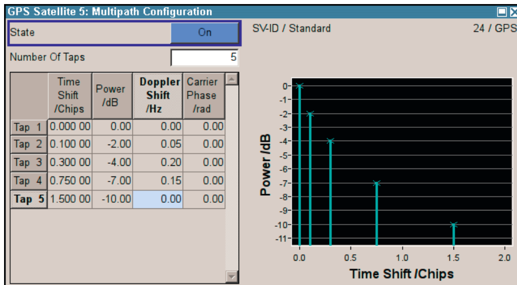
The R&S®SMBV100A allows several multipath taps per satellite to be defined.
