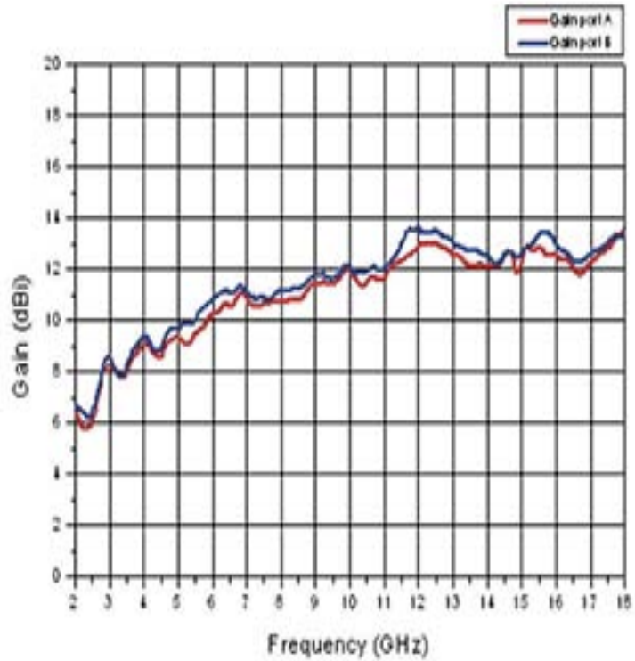
Model 3164-05 Open Boundary Quad-Ridged Horn Gain (measured per SAE 958 Rev. C)
