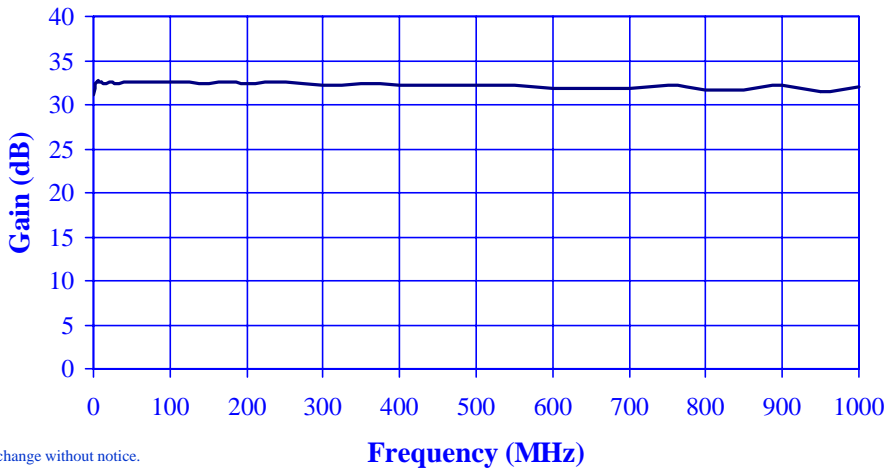
Typical Gain model PA-103
