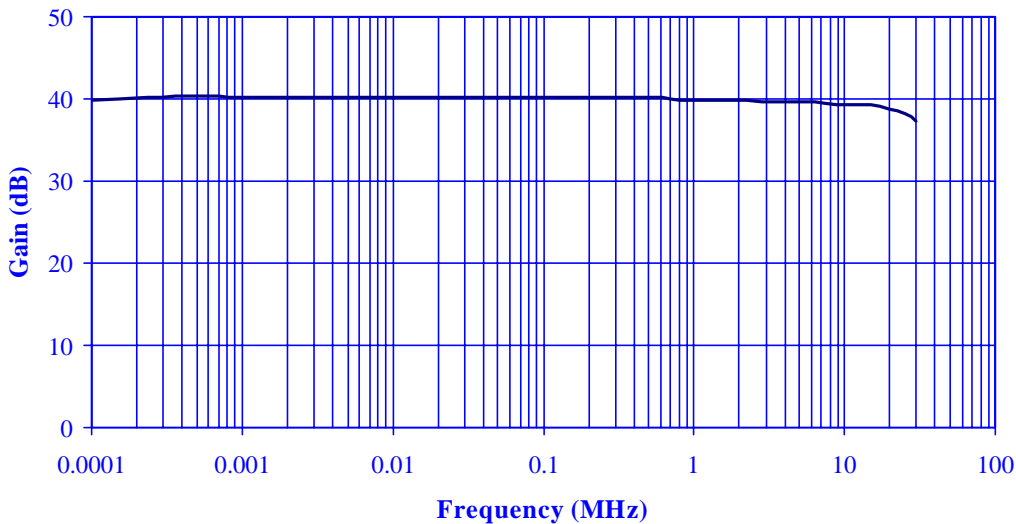
Typical Gain model PA-103
