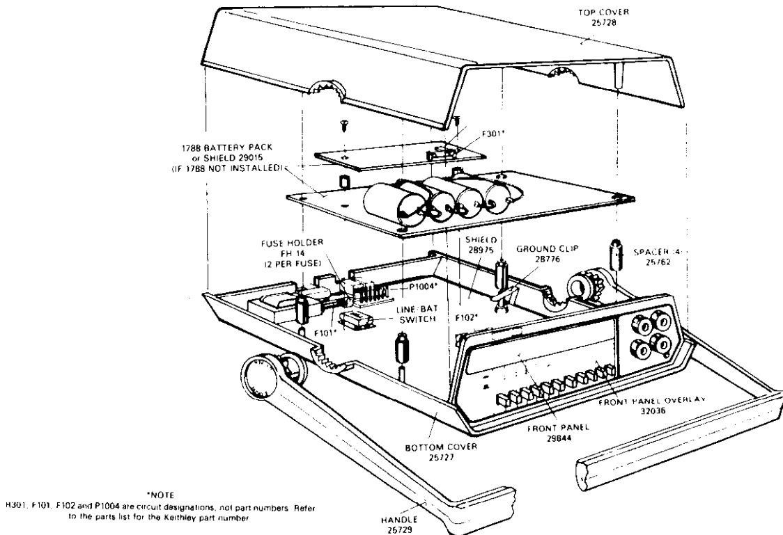
Figure 6-1. Miscellaneous Parts
